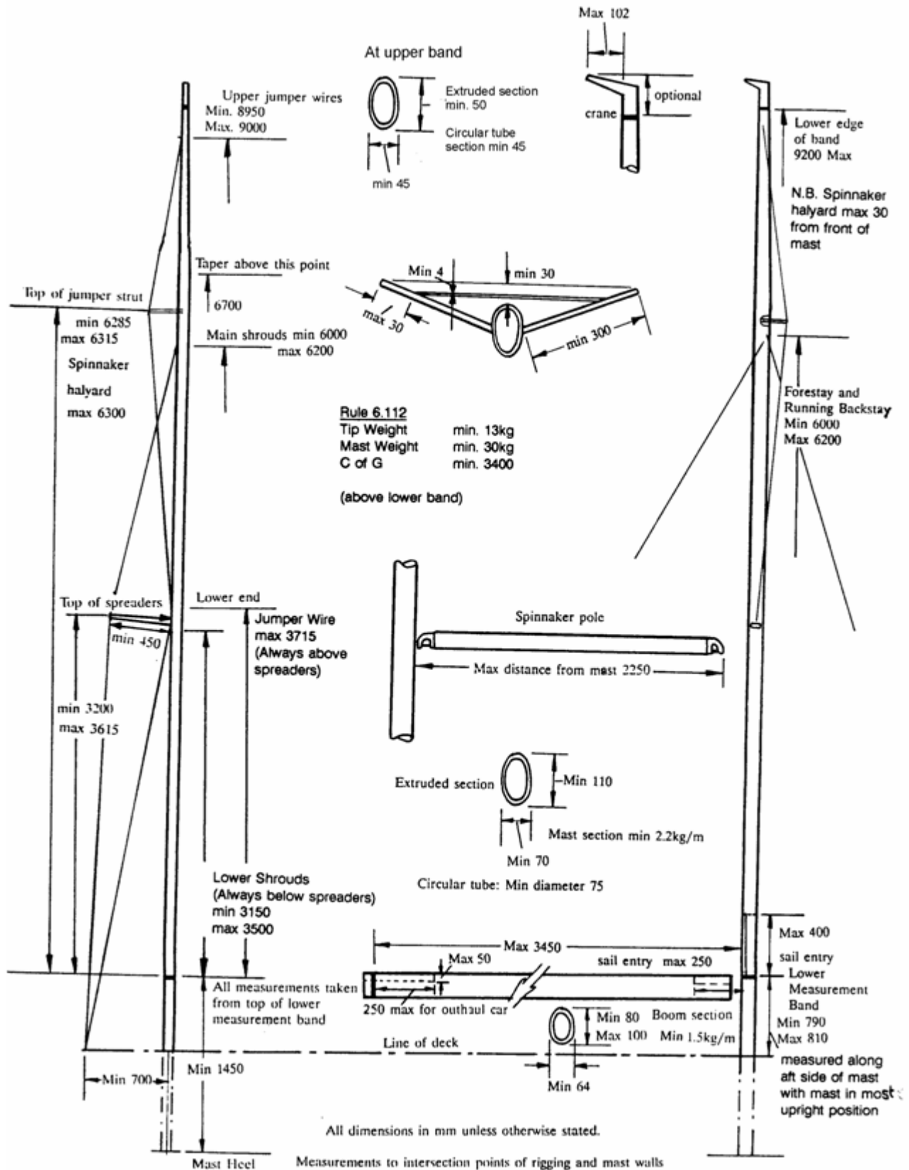
DIAGRAM OF SPARS
